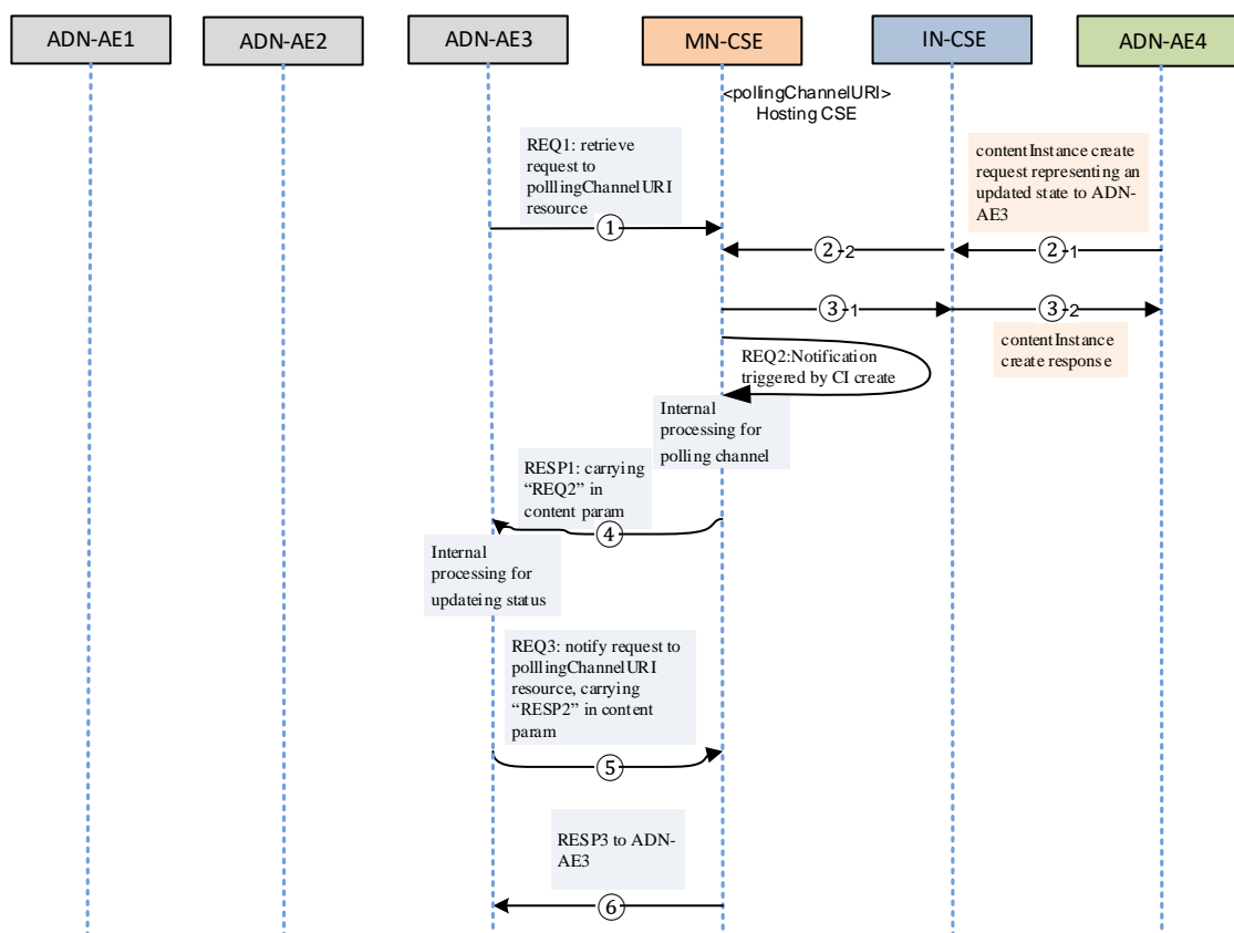
Figure 7.2.5-1: Actuator remote control phase call flows
